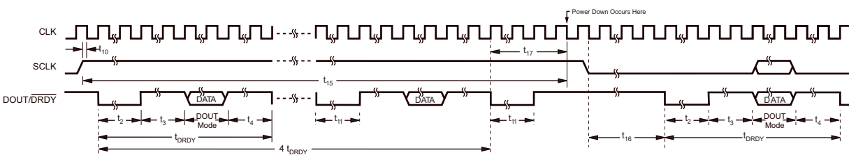
Figure 35. Power-Down Mode
